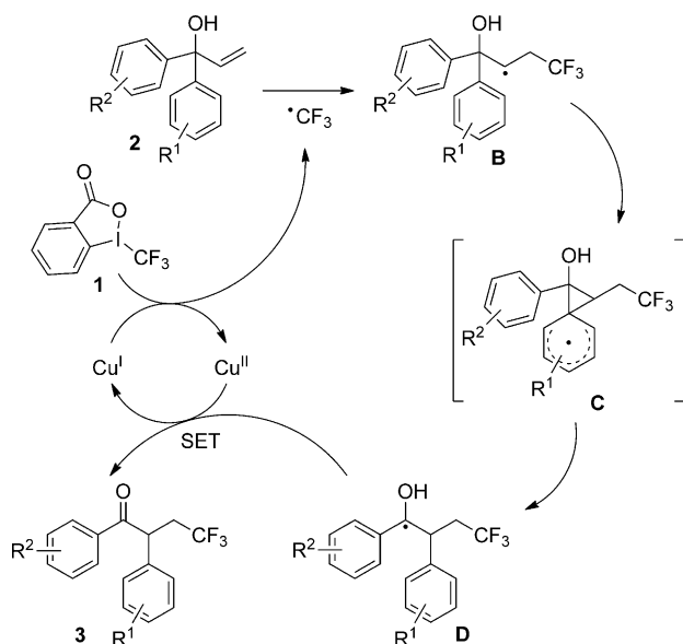
Scheme 3. The proposed mechanism for Cu-catalyzed trifluoromethylation-initiated radical 1,2-aryl migration in \alpha,\alpha -diaryl allylic alcohols.
