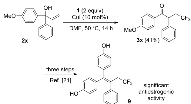
Scheme 2. Formal synthesis of antiestrogenic compound 9 .
