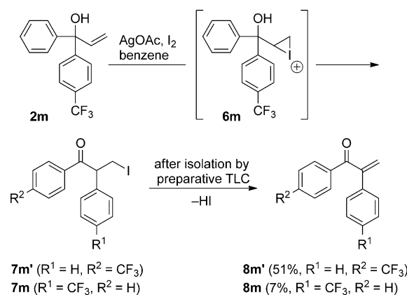
Scheme 1. Opposite chemoselectivity for rearrangement of 2m under Ciganek's conditions.
